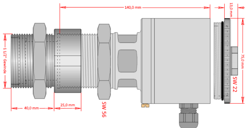
Fig. 2 Microwave sensor
