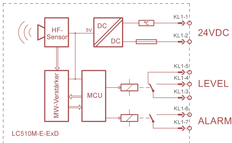
Fig. 6 receiver LC510M-E-ExD
