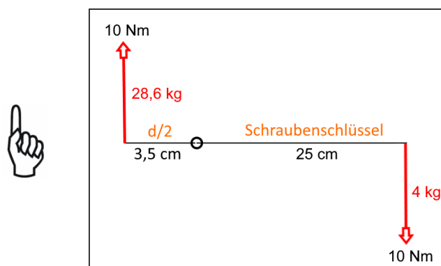
Fig. 8 Minimum torque with a wrench
