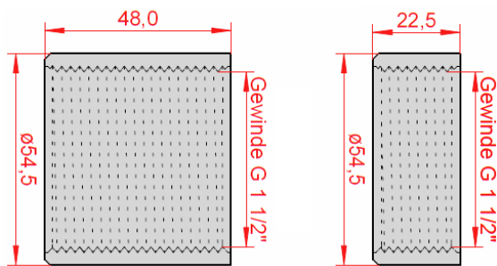
Fig. 9 Dimensions of the Cylinder sleeve
