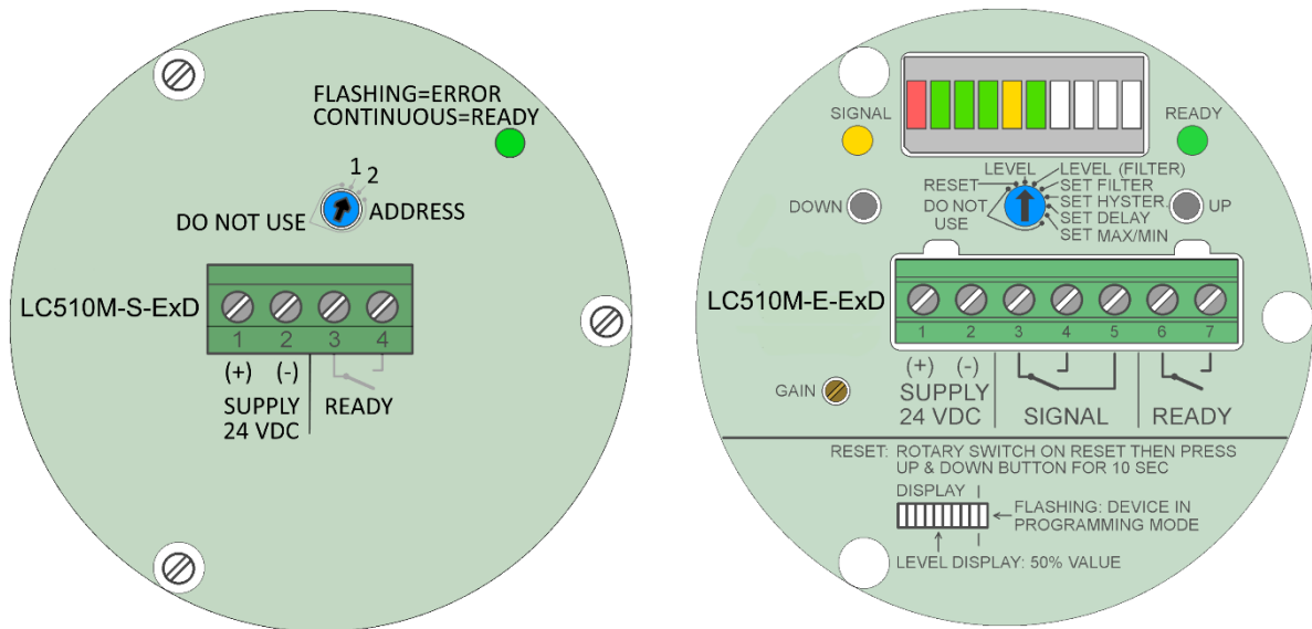
Fig. 12 Illustration of all operating and display elements of the MW transmitter and MW receiver
